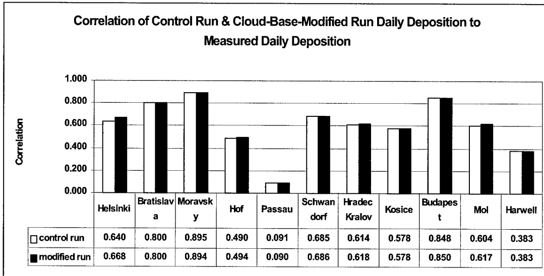
Figure 64 Set 1. Pearson correlation coefficients of modeled Chernobyl Cs-137 daily deposition (control run and modified-cloud-base run) against measured Chernobyl Cs-137 daily deposition, by city. In order by earliest deposition measurement at each city.
