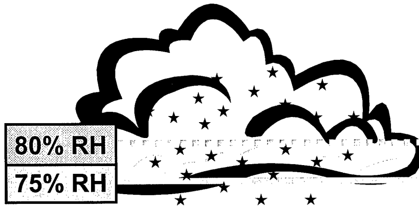
Figure 3 Illustration of cloud representation in HYSPLIT. Stars represent pollutant plume. 80% RH is the default cloud base, 75% RH is the tested modification.
