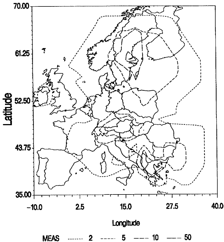
Figure 2 Geographic plot of contours of accumulated Cs-137 deposition [ kBq/m^2 ] from 27Apr1986 to 10May1986. ATMES Report Figure 10 (Klug 92).
