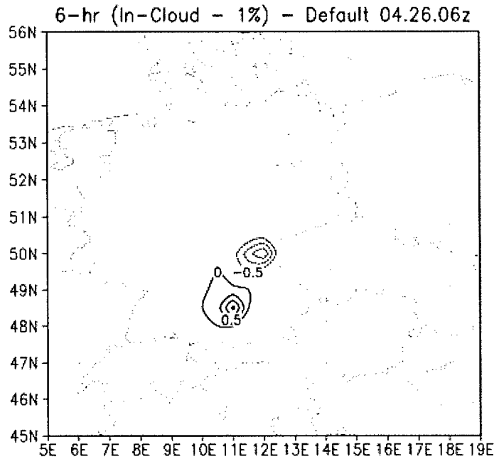
Figure 24 Difference in 6-hr-accumulated Cs-137 deposition [ Bq/m^2 ]; Deposition from a test run with a 1% reduction of in-cloud scavenging efficiency less deposition from control run, 86.04.26.06Z
