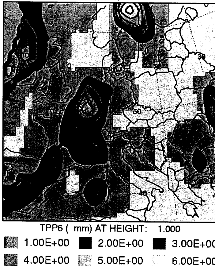
Figure 21 Reanalyzed ECMWF model precipitation in [mm] accumulated from 86.04.26.00Z to 86.04.26.06Z for comparison to in-cloud scavenging sensitivity run. Contours in 1-mm increments.
