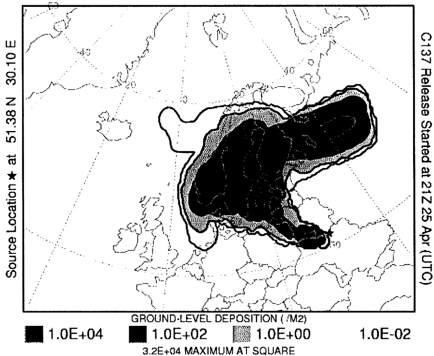
Figure 6 Attempted duplicate of ARL's Chernobyl Cs-137 deposition. Source modeled as uniform vertical line source from 750m to 1500m at a rate of 10^{15} Bq/hr for 24 hours. Deposition velocity set at 0.1cm/s. In-cloud scavenging ratio set at 3.2 \times 10^5 l/l . Below-cloud scavenging rate set at 5.0 \times 10^{-5} s^{-1} . Deposition contoured on a logarithmic scale.
